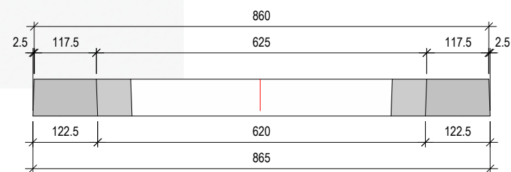
Section on Cut Line B - B
