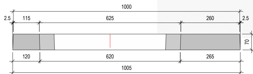
Section on Cut Line A - A
