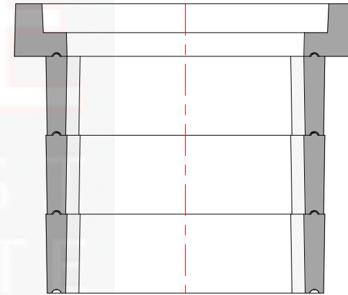
Typical Section Through 600mm x 450mm HIC Chamber & Frame
