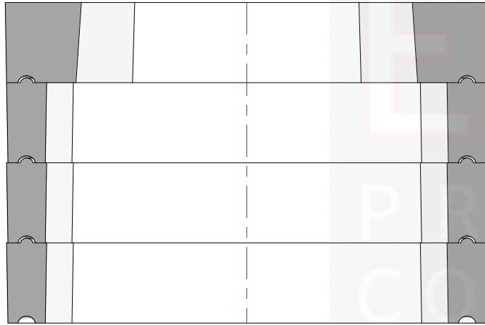
Typical Section Through 1200mm x 750mm HIC Chamber & Heavy Duty Lid
