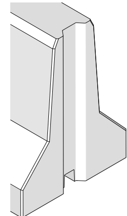
Typical Chamfer Detail scale 1:15
