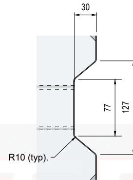
Female Connection scale 1:5
