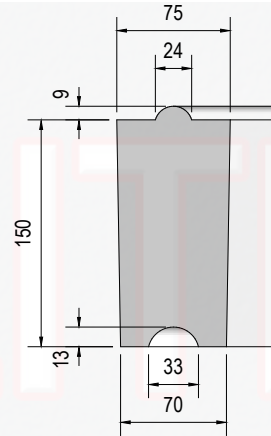
Section Profile (scale 1:5)
