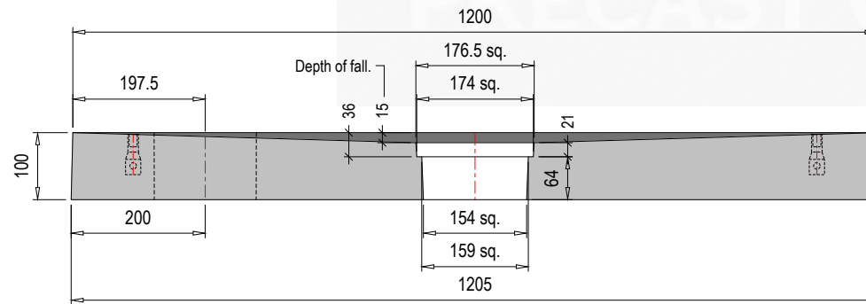
Part Section on Arrow A - A
