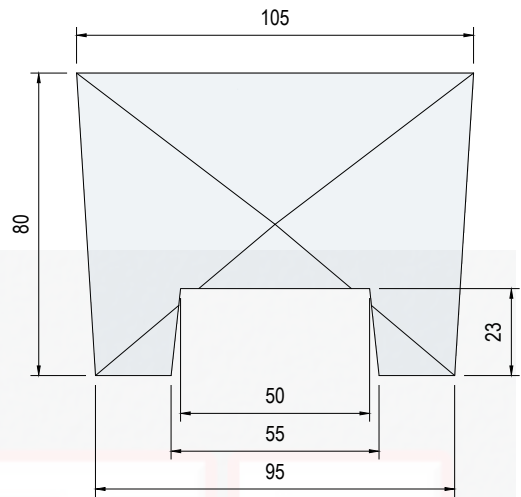
Cross Sectional Detail (scale 1:2)
