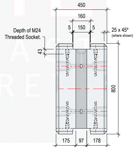
Part Section on Arrow A - A Detail Identical Both Ends
