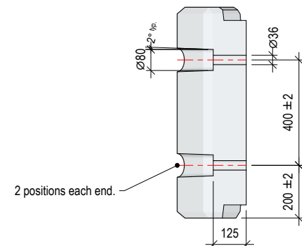
Part Section on Arrow A - A Detail Identical Both Ends
