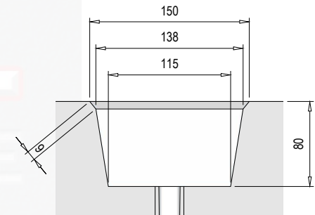
Post Mounting Hole Detail (scale 1:5)
