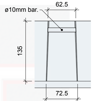
Lifting Point Detail (scale 1:5)
