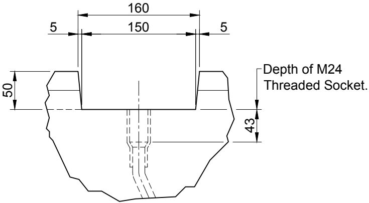
Channel Detail Scale 1:5
