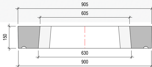
Part Section on Arrow B - B
