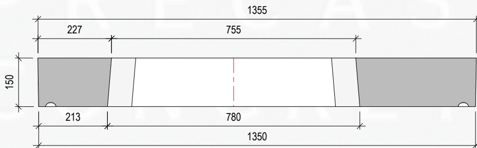
Part Section on Arrow A - A
