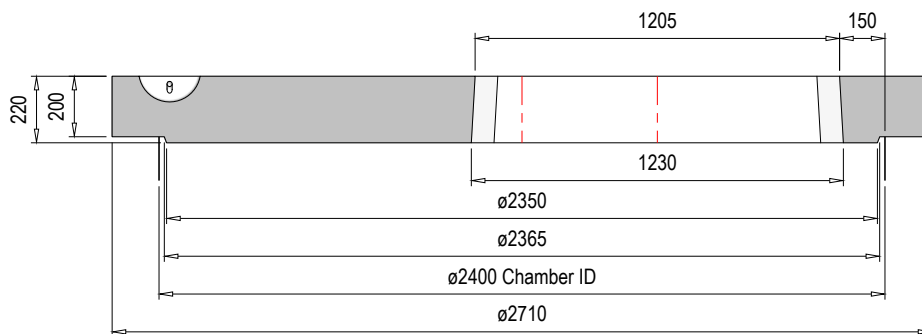
Part Section on Arrow A - A
