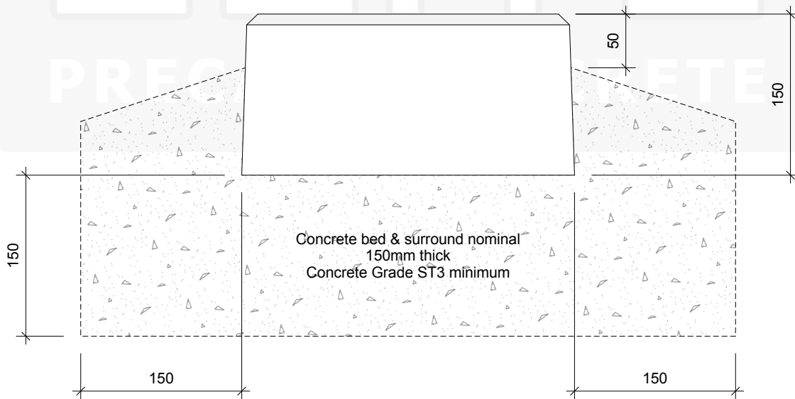
Typical Installation Detail
