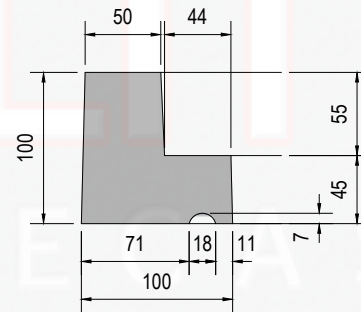
Section Profile (scale 1:5)
