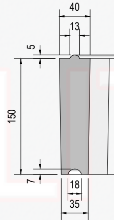
Section Profile (scale 1:5)
