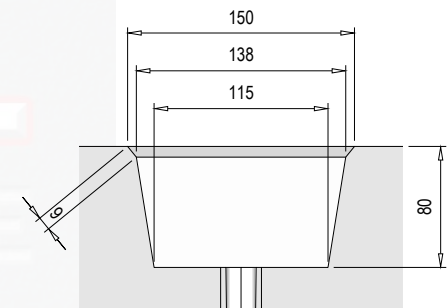
Post Mounting Hole Detail (scale 1:5)
