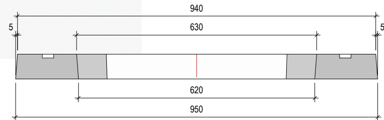
Section on Cut Line B - B
