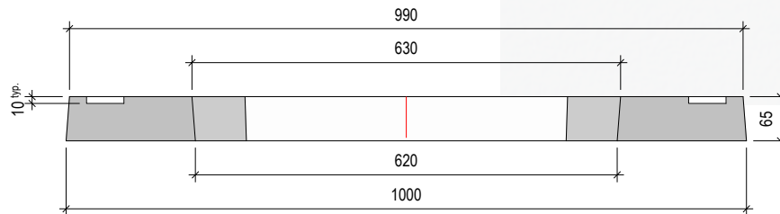
Section on Cut Line A - A
